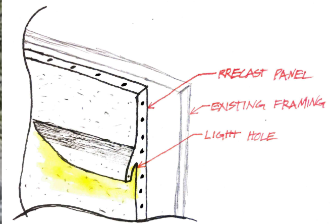
PERSPECTIVE DETAIL
